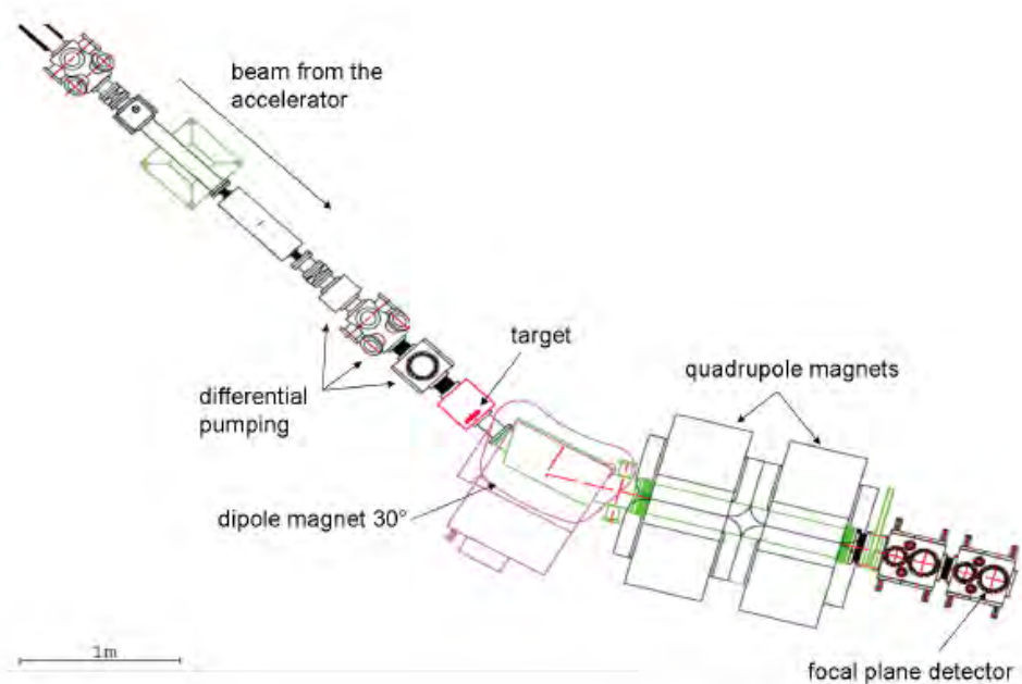
Fig. 2.6: Schematic drawing of TASCA.
