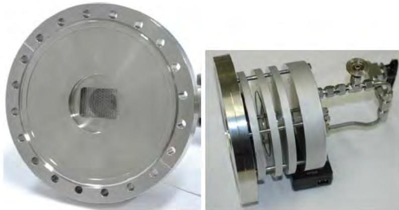
Fig. 2.15: Left: The SIM RTC with an entrance window of 30 \times 40 \text{ mm}^2 . Right: Side view of the SIM RTC. Spacers can modularly be introduced to the setup to change the depth of the RTC.
