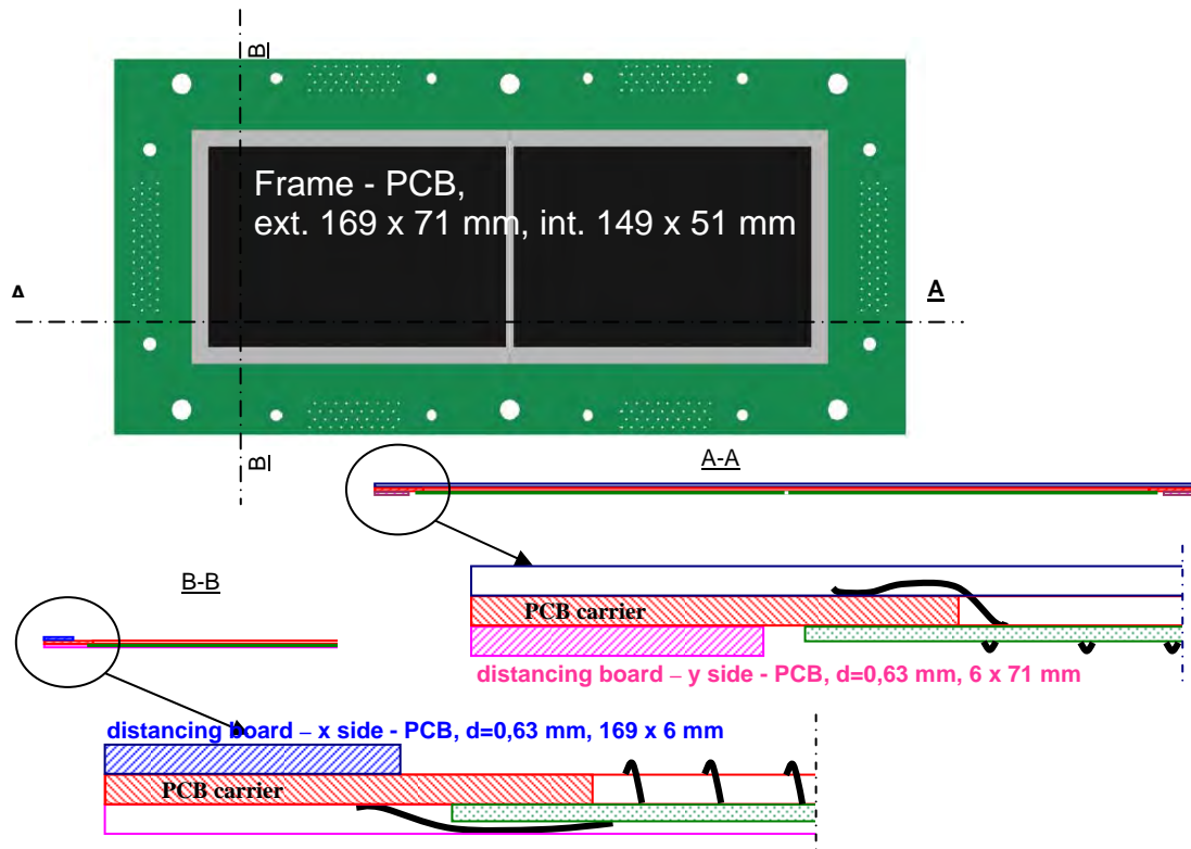
Fig. 5.2: Implantation detector frame and wire bonding.
