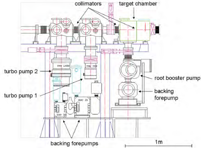
Fig. 2.7: Technical drawing of the differential pumping system of TASCA. The gas collimators have the following diameters: C_1 = 10 mm, C_2 = 13 mm, C_3 = 18 mm (from right to left).
