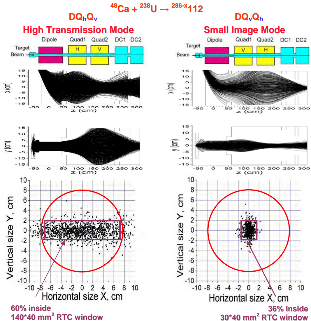
Fig. 2.12: The two final ion-optic TASCA configurations: (a) SIM and (b) HTM.
