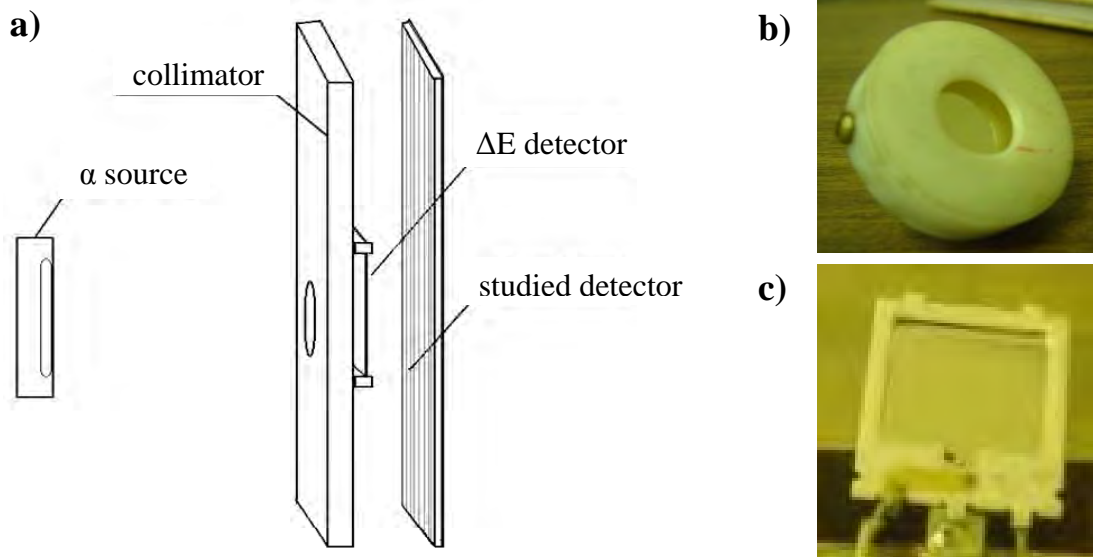
Fig. 5.6. Schematic view of test stand (a), ^{238}\text{Pu} \alpha -source (b) and 10 \mu\text{m} thick \Delta E detector (c).
