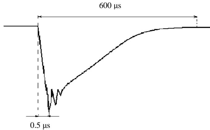
Fig. 5.7. Typical form of the signal from the tested DSSSD detector.
