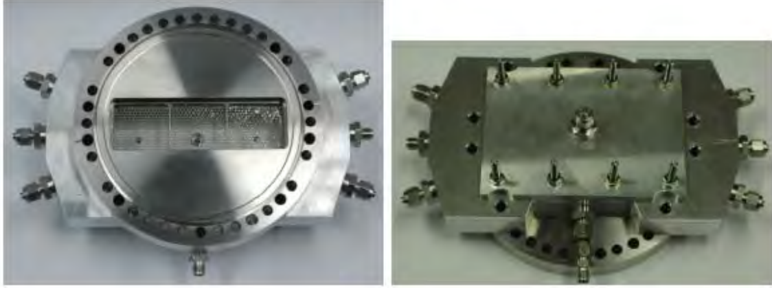
Fig. 2.14: Left: The HTM RTC viewed from the side which is attached to the separator. The supporting honeycomb structure 140 \times 40 \text{ mm}^2 can be seen. Right: HTM RTC from the other side, the many gas valves for an adjustable gas flow are visible.
