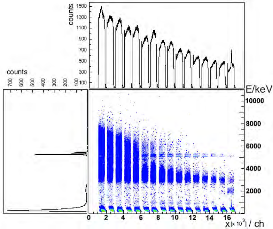
Fig. 3.11: Energy over horizontal position spectrum for all 16 strips of the PSSSD. Each point within the central plot represents one event. Position is defined as: (strip number \times 1000 + position in the strip) and the energies are in keV. The integral distributions are plotted on the sides.
