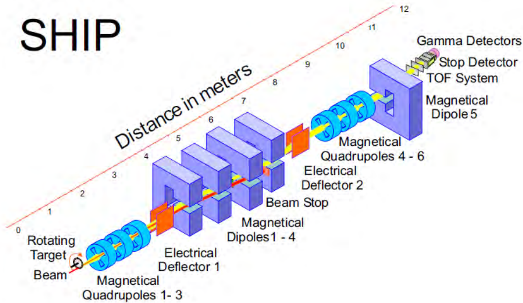
Fig. 2.2: Schematic drawing of SHIP separator with the coupler at the end of its detection system.
