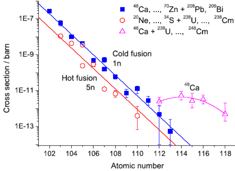
Fig. 1.12: Experimental cross sections for the formation of nuclei with Z \geq 102 in (■) the 1n evaporation channel of cold fusion reactions, (○) the 5n channel of hot fusion reactions, and (Δ) the fusion reaction with the ^{48}\text{Ca} + actinide targets. The curves are drawn to guide the eye. Adapted from [50].
