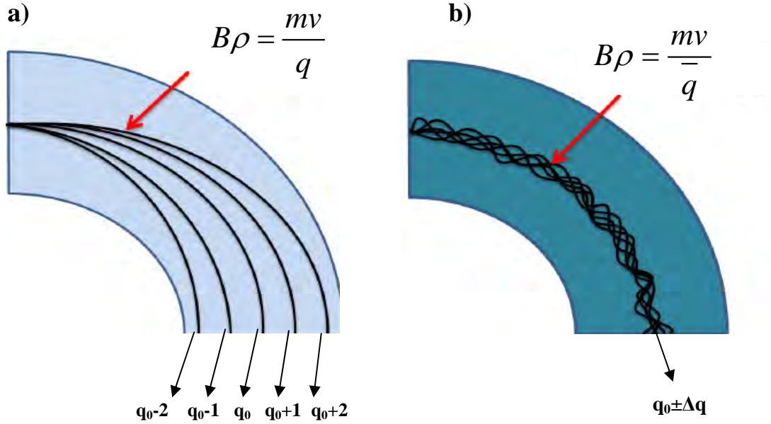
Fig. 2.3: Magnetic rigidities of heavy ions a) in vacuum and b) in He gas. In the gas-filled magnetic field region, the discrete trajectories corresponding to the different charge states collapse around a trajectory defined by the average charge state of the ion in the gas.
