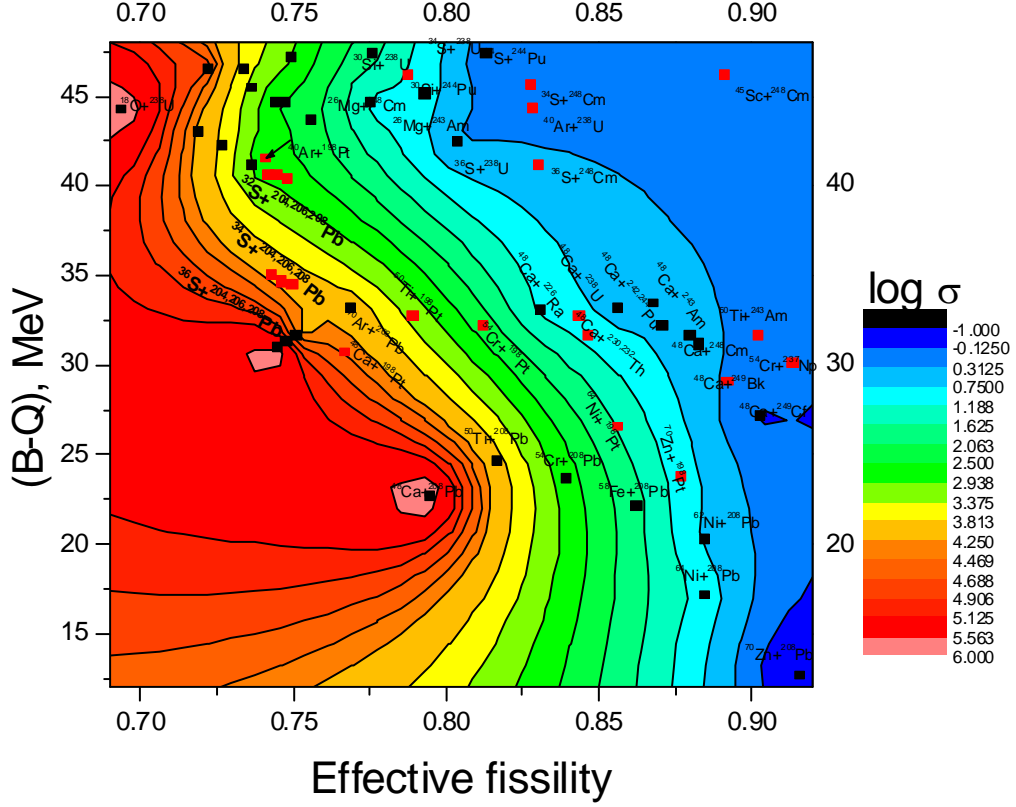
Fig. 1.16: Contour plot showing the correlation of the evaporation residue cross section from the fissility and the (B - Q) parameter. Adopted from [50].
