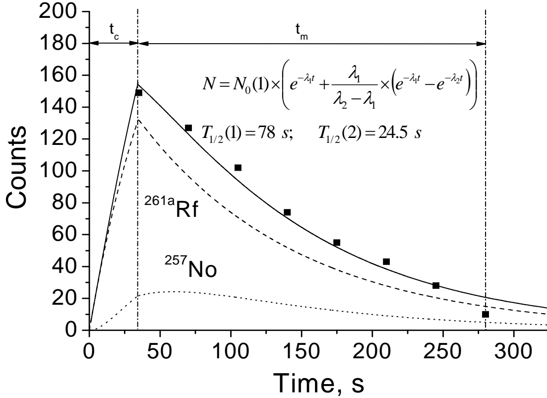
Fig. 4.6: The production and the decay curves for ^{261\text{a}}\text{Rf} ( T_{1/2} = 78 s, dashed line), its daughter ^{257}\text{No} ( T_{1/2} = 24.5 s, dotted line) and the sum of both (solid line). Symbols represent numbers of surviving ^{261\text{a}}\text{Rf} + ^{257}\text{No} nuclei starting from the beginning of the measurement ( t = 35 s). Time intervals t_c and t_m represent the collection time and measurement time, respectively.
