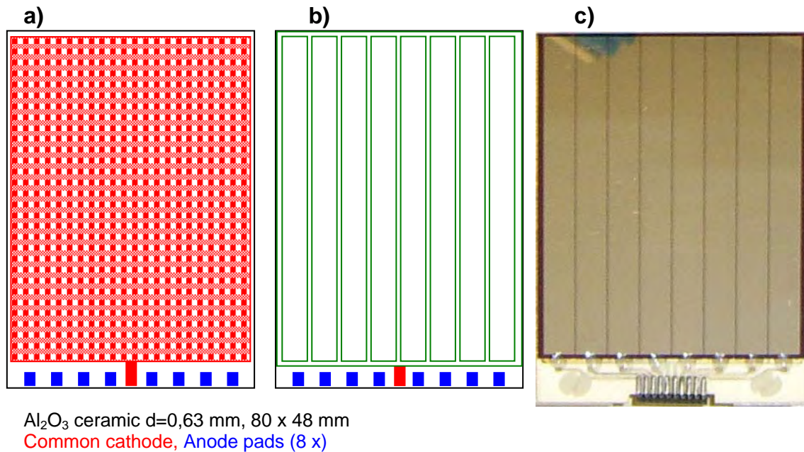
Fig. 5.4: SSSSD detector: a) \text{Al}_2\text{O}_3 ceramic plate with common contact, b) schematic view of the SSSSD detector and c) photo of the finished device.
